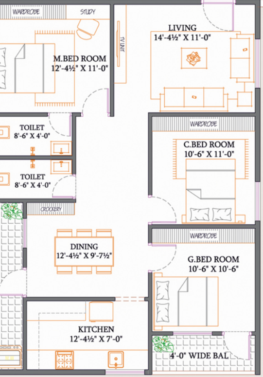
Area - 1340 Sft.
