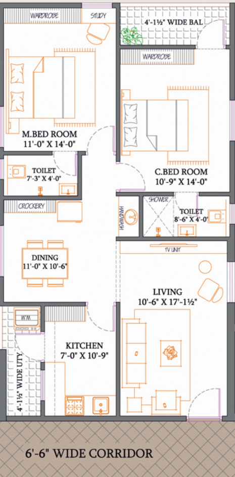
Area - 1180 Sft.
