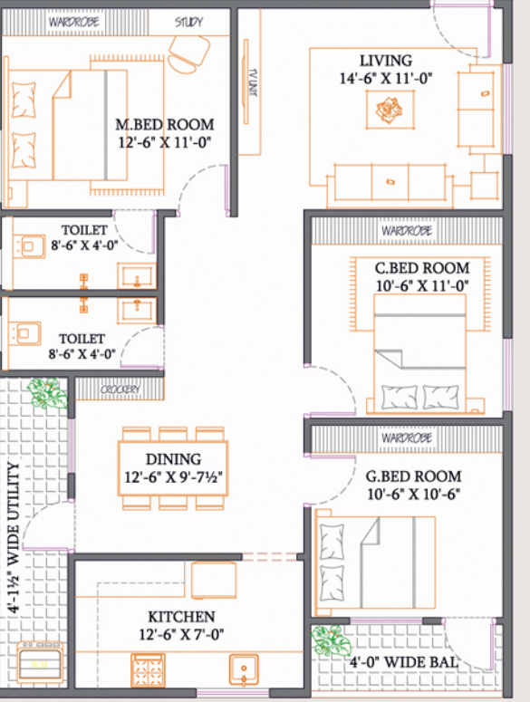
Area - 1350 Sft.
