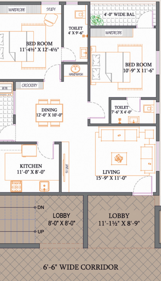
Area - 1130 Sft.
