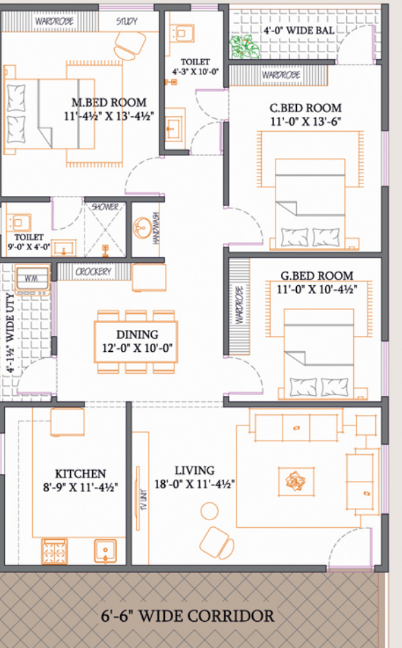
Area - 1450 Sft.
