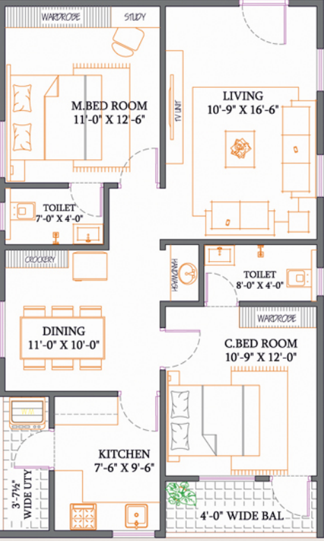
Area - 1100 Sft.
