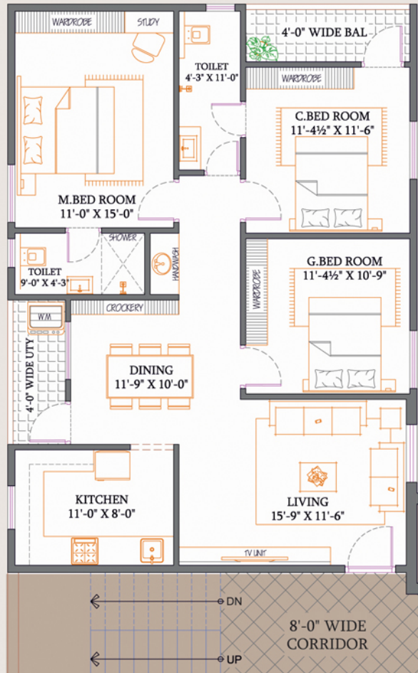
Area - 1400 Sft.
