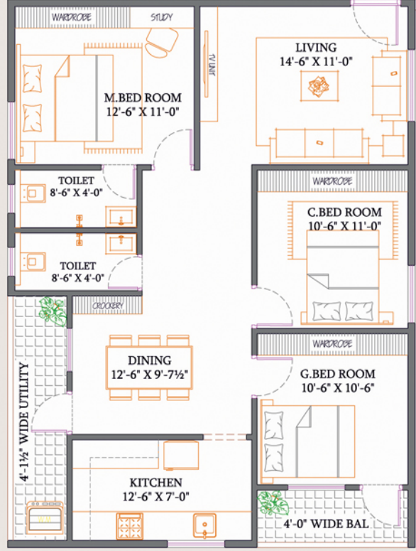
Area - 1350 Sft.
